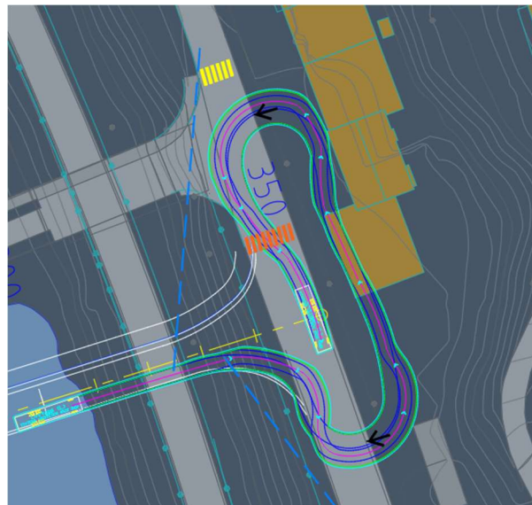
Figur 1-14 Kryssing for gående
